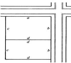
Lot Lines: (a) Corner Side Yard Line (b) Front Yard Line (c) Rear Yard Line (d) Side Yard Line
