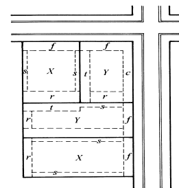
Transition Yards (T)
