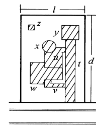
Lot Coverage (m)
